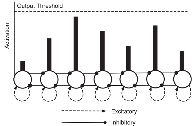
Figure 2. A schematic of the lateral inhibition neural network architecture employed for the simulations. The network is modeled on the competitive choice layer employed in competitive queuing models of serial behavior (Bullock, 2004; Bullock & Rhodes, 2003). Each localist item node possesses a single recurrent excitatory connection, as well as lateral inhibitory connections to all other item nodes. Nodes are fully interconnected, but only adjacent-neighbor inhibitory connections are shown to prevent visual cluttering. The activation of a node within the layer is determined by the external input it receives from outside the layer, plus positive recurrent self-excitation, and within-layer lateral inhibition. The number of nodes in the network is dependent on the sequence length being modeled.
